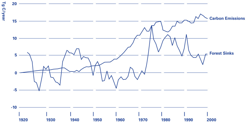
Carbon Emissions & Forest Carbon Sinks 1920-2000
